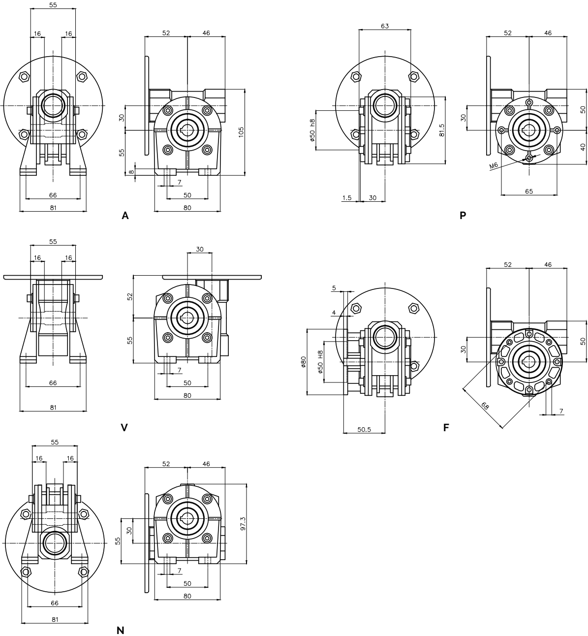
Gearbox Dimensions
